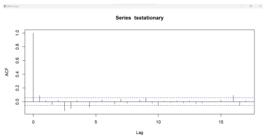
Fig. 8. Autocorrelation Function Diagram
