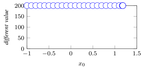
Fig. 7: Input x_0 in function x_i = x_{i-1}^2 - 1 + \frac{2}{3x_{i-1}}
