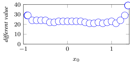
Fig. 13: Input x_0 in function x_{n+1} = \sqrt{x + 1 - \frac{2}{3x}}
