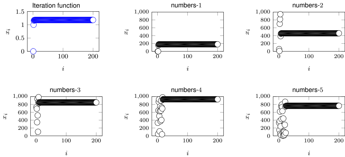
Fig. 12: Results of the First 200 Iterations of the Function x_{n+1} = \sqrt{x + 1 - \frac{2}{3x}}
