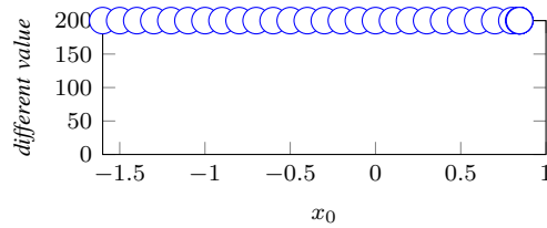
Fig. 11: Input x_0 in function x_{n+1} = 1 + \frac{1}{x} - \frac{2}{3x^2}
