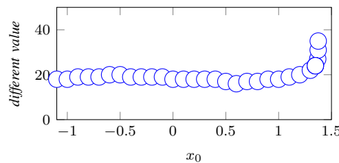
Fig. 9: Input x_0 to the Function x_{i+1} = \sqrt{x_i^3 - x_i + \frac{2}{3}}
