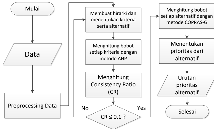
Fig. 2. Flowchart Sistem
