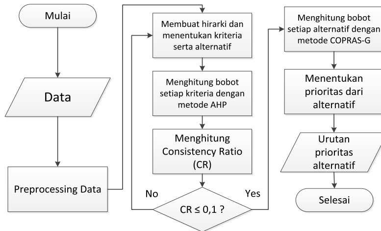
Gambar 2 Flowchart Sistem
